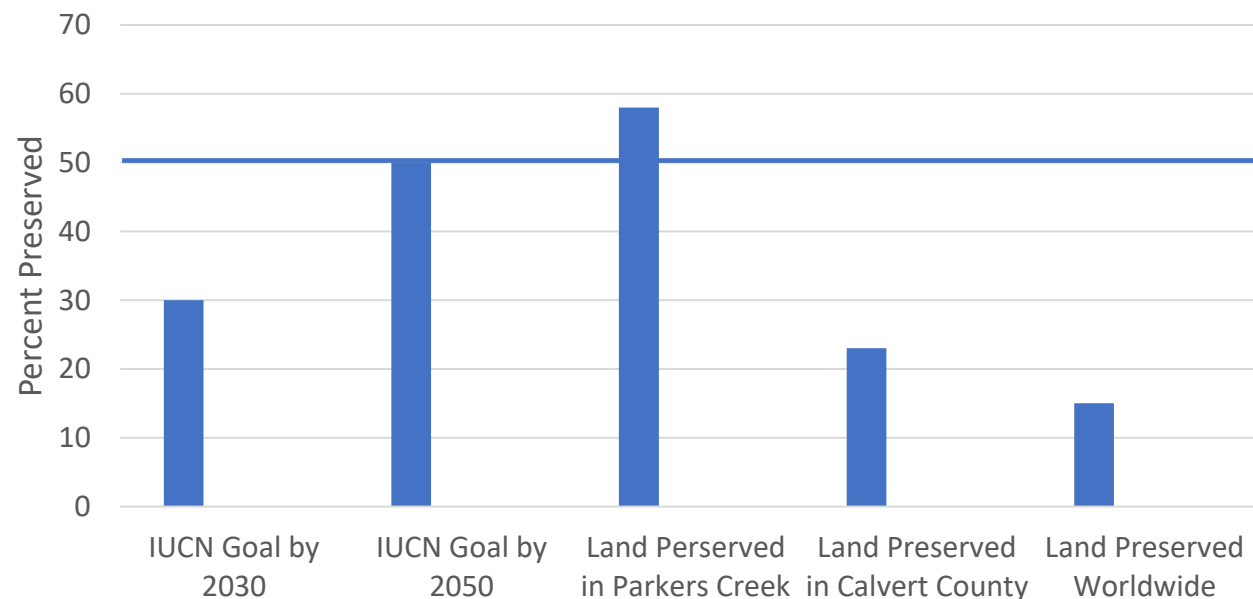
Percent of Land Preserved Recommendations vs Actual
